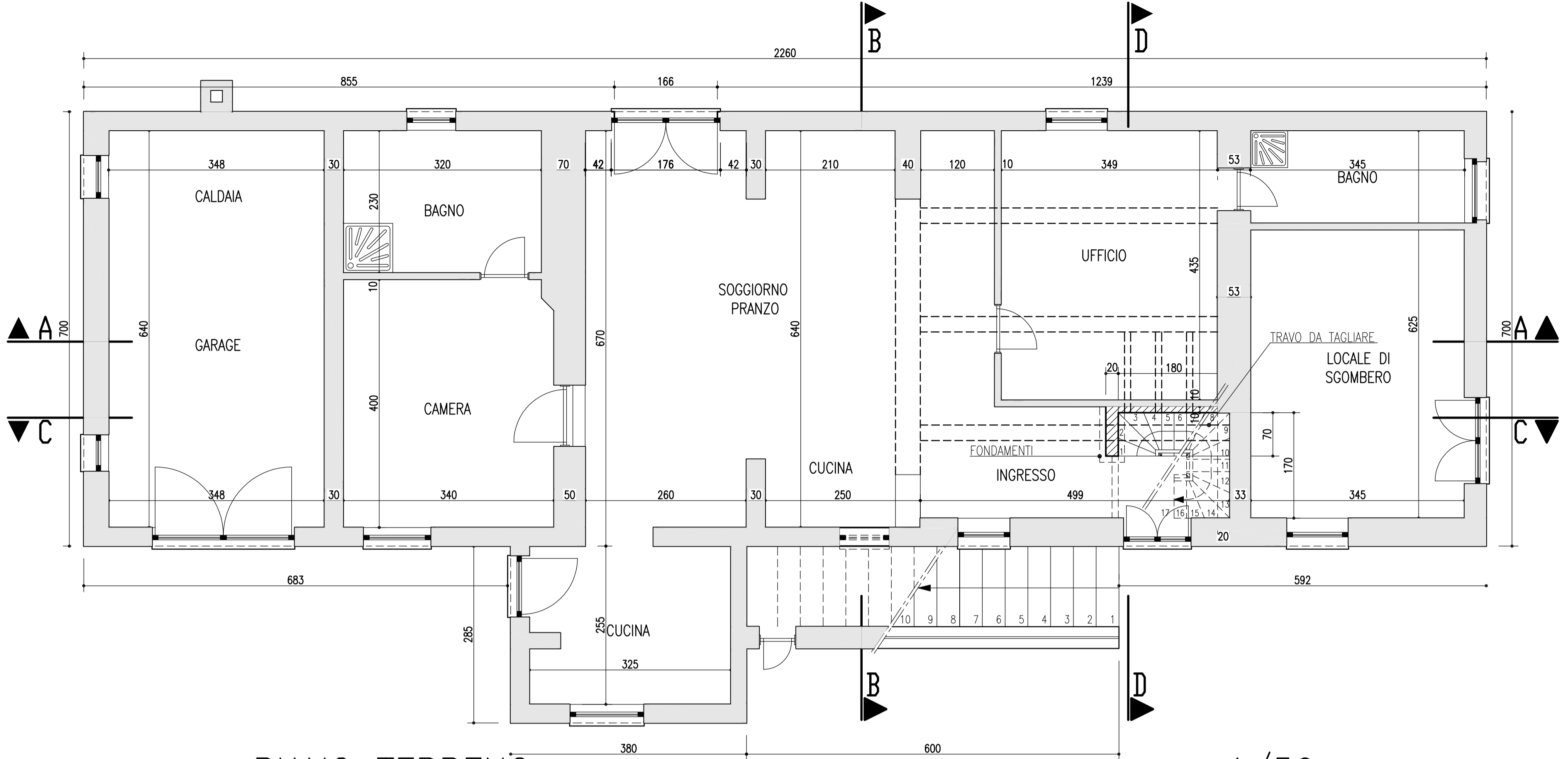
PIANO TERRENO
