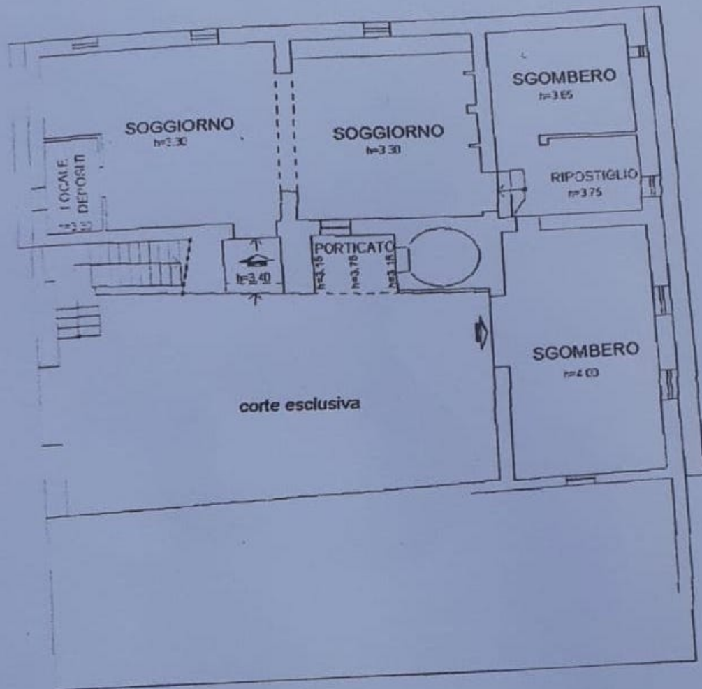
PIANO TERRA
